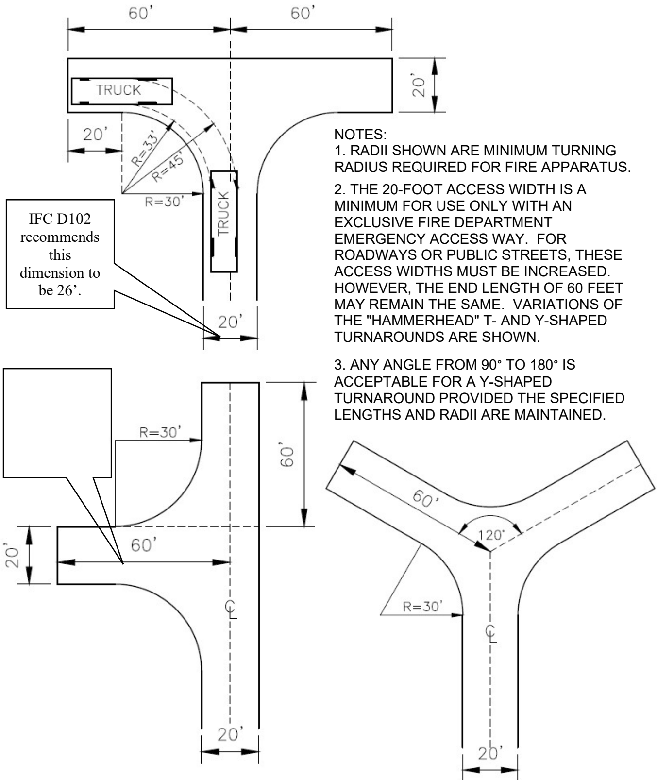
FIGURE II-8: T- AND Y-SHAPED TURNAROUND DIMENSIONS
