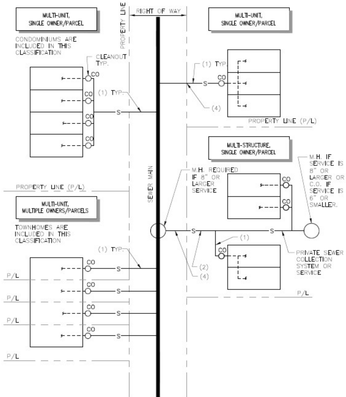
FIGURE III- 8: TYPICAL SANITARY SEWER SERVICE LINE LAYOUTS
