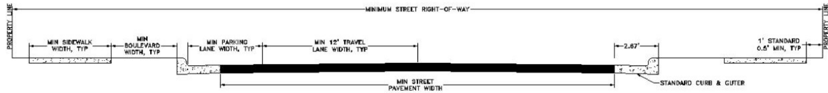
FIGURE II-9: STREET AND RIGHT-OF-WAY CRITERIA
